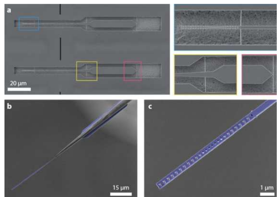
Top-left: Scanning electron micrograph top-view of two fabricated devices on a silicon on insulator chip. Right: Zoom-ins of the boxed regions; b) False colour scanning electron microscope image showing the silicon superfluid wave flume (blue) glued to a silica optical fibre taper (grey); c) Zoomed-in view showing the silicon photonic crystal cavity at the end of the device. The silicon waveguide is around 500 nm wide and 220 nm thick. ARXIV:2504.13001V1
